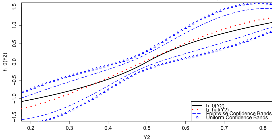
Figure 1: Model in Experiment 2 95% Pointwise Bands and Uniform Bands of h_0(Y_2)
