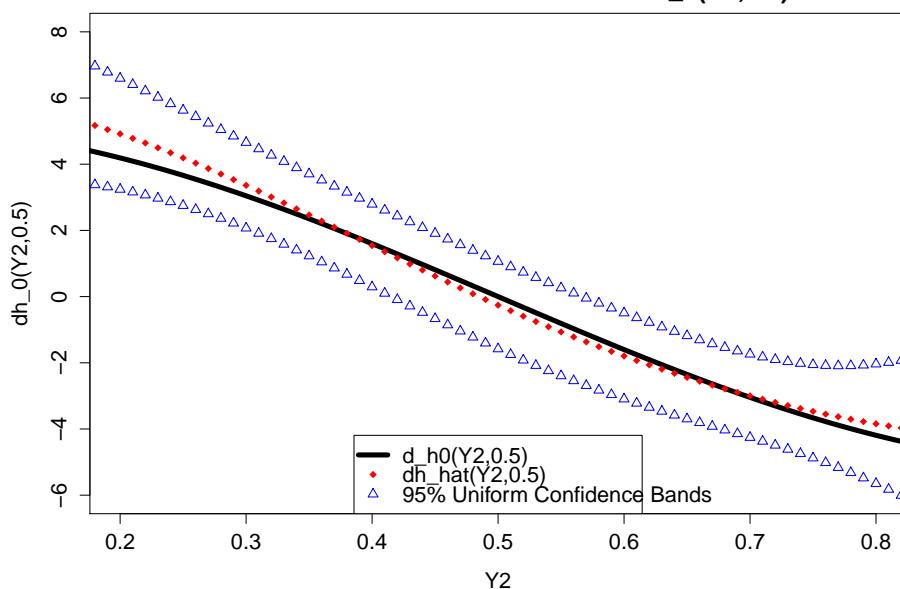
Figure 2: Model in Experiment 3 95% Uniform Confidence Bands of dh_0(Y2,0.5)
