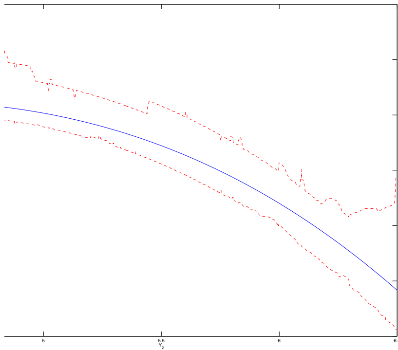
Figure 6.2: PSMD Estimate of the NPQIV food-in Engel curve (blue solid line), with the 95% pointwise confidence bands (red dash lines).
