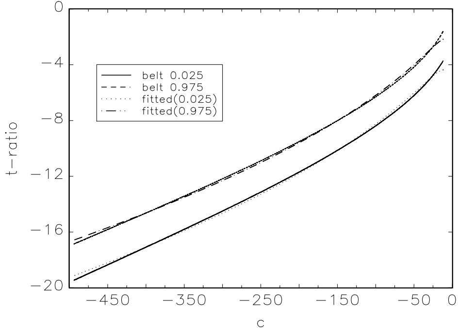
Fig. 1: Confidence belts (at levels 2.5% and 97.5%) based on local to unity ( \rho = 1 + \frac{c}{n} ) limit theory for the t ratio t_{\hat{\rho}} = \frac{\hat{\rho} - 1}{\hat{\sigma}_{\hat{\rho}}} , shown against fitted regression curves of the form f(c) = \alpha_0 + \alpha_1 |c|^{1/2} + \alpha_2 |c|^{-1/2} , as suggested by the asymptotic functional form of the belts given in (13).
