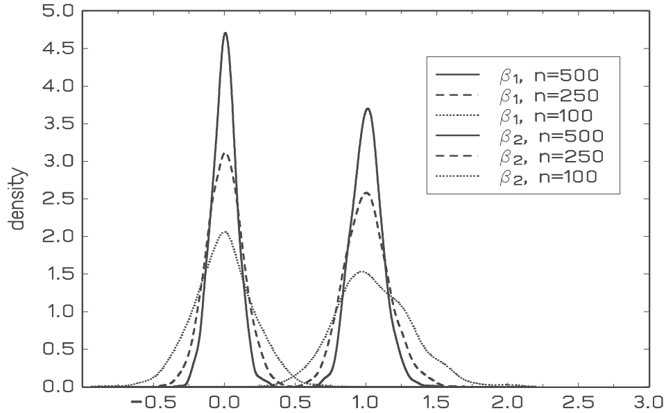
Figure 3: Logit Model - densities of estimators of \beta_1^0 = 1 , \beta_2^0 = 0 ; Stationary case
