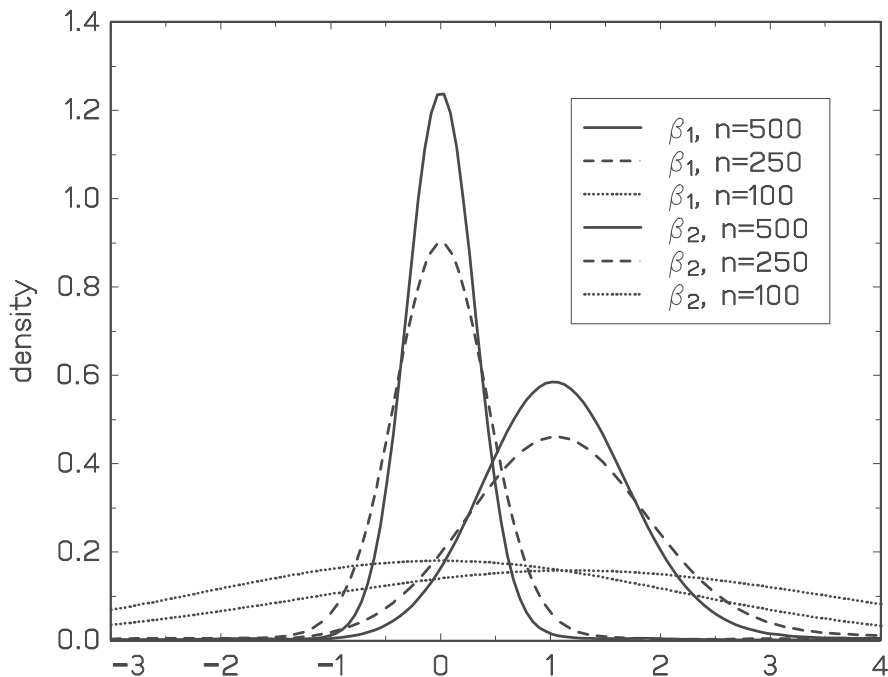
Figure 2: Probit Model - densities of estimators of \beta_1^0 = 1, \beta_2^0 = 0 ; I(1) case.
