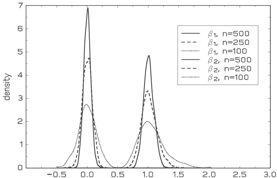
Figure 4: Probit Model - densities of estimators of \beta_1^0 = 1 , \beta_2^0 = 0 ; Stationary case.
