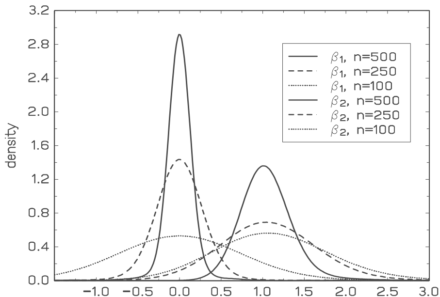
Figure 1: Logit Model - densities of estimators of \beta_1^0 = 1 , \beta_2^0 = 0 ; I(1) case.
