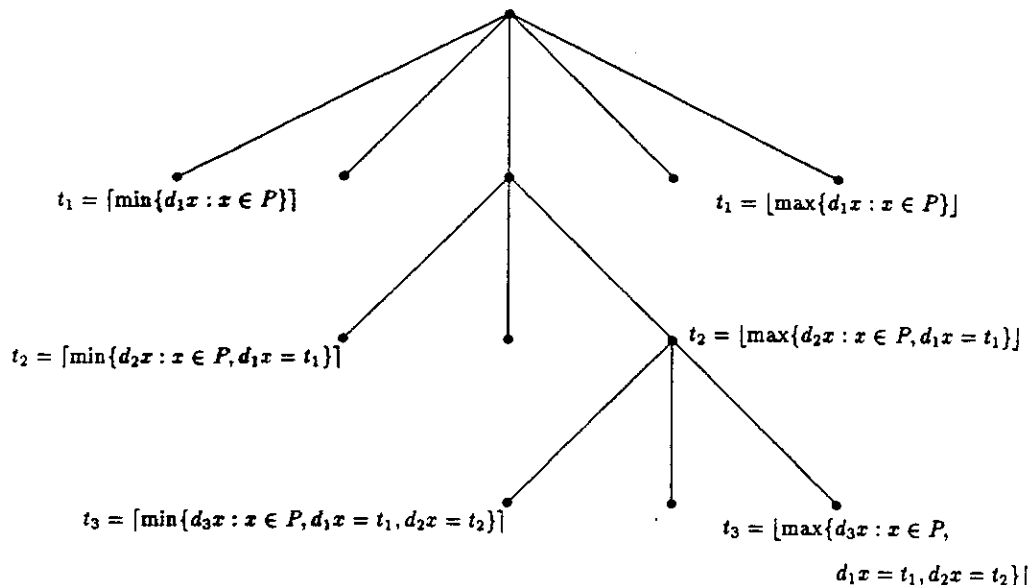
Figure 1: Search tree
