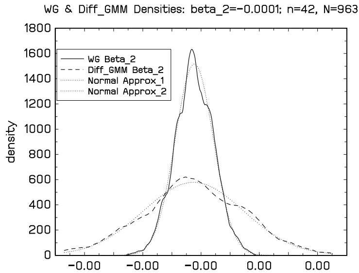
Figure 8: Kernel estimates of the densities of WG and diff-GMM estimates of \beta_2 based on R = 1500 replications with n = 42, N = 963 , and true value \beta_2 = -0.0001 .
