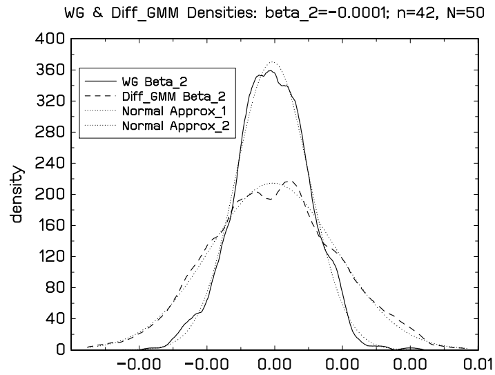
Figure 4: Kernel estimates of the densities of WG and diff-GMM estimates of \beta_2 based on R = 1500 replications with n = 42, N = 50 , and true value \beta_2 = -0.0001 .
