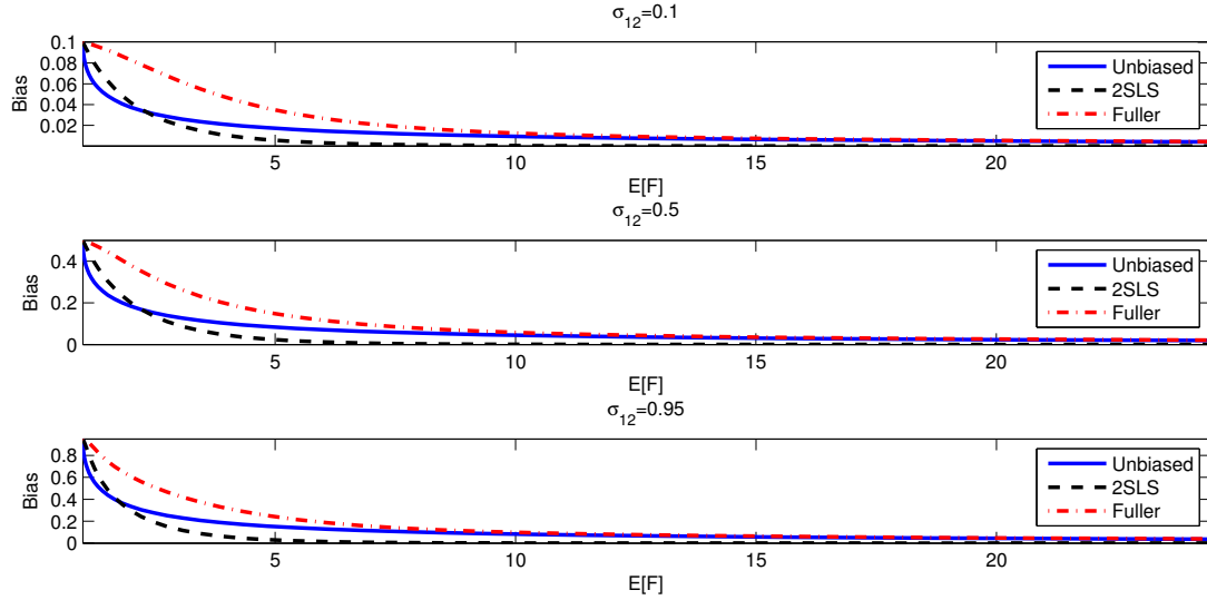
Figure 8: Median bias of single-instrument estimators, plotted against mean E[F] of first-stage F-statistic, based on 10 million simulations.
