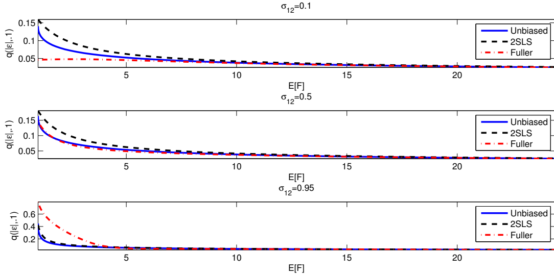
Figure 9: Tenth Percentile of |\varepsilon| = |\hat{\beta} - \beta| for single-instrument IV estimators, plotted against mean E_{\pi} [F] of first-stage F-statistic, based on 10 million simulations.
