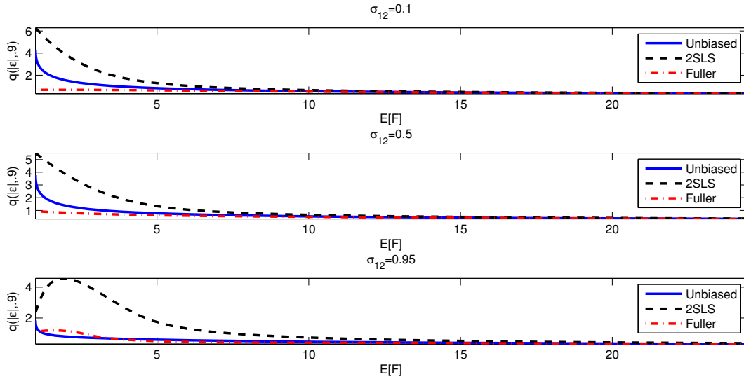
Figure 10: Ninetieth Percentile of |\varepsilon| = |\hat{\beta} - \beta| for single-instrument IV estimators, plotted against mean E_{\pi} [F] of first-stage F-statistic, based on 10 million simulations.
