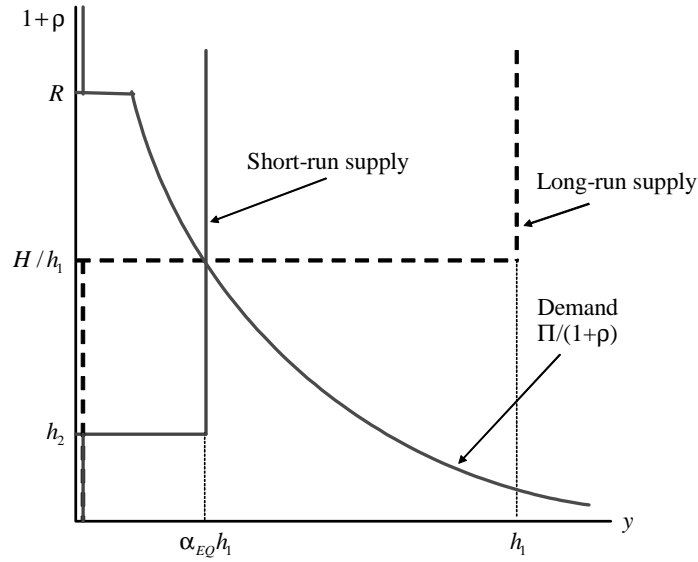
Figure 5. Equilibrium in the Case \Pi < h_1 h_2
