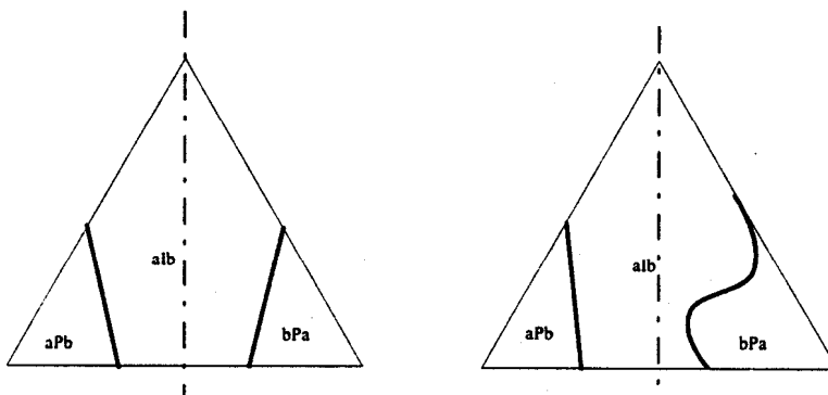
Figure 3. Examples of a SWFs that satisfies Neutrality (left) and fails Neutrality (right).
