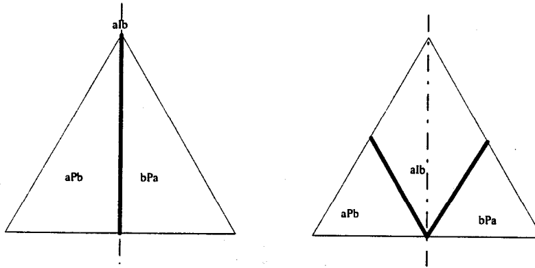
Figure 4. Majority Rule (left) and Strict Majority Rule (right)
