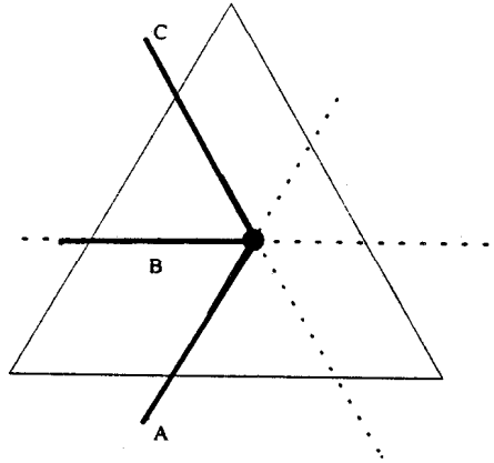
Figure 6. Illustration of monotonicity axioms
