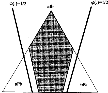
Figure 10. A SWF where \varphi -Weak I -Mon does not bite
