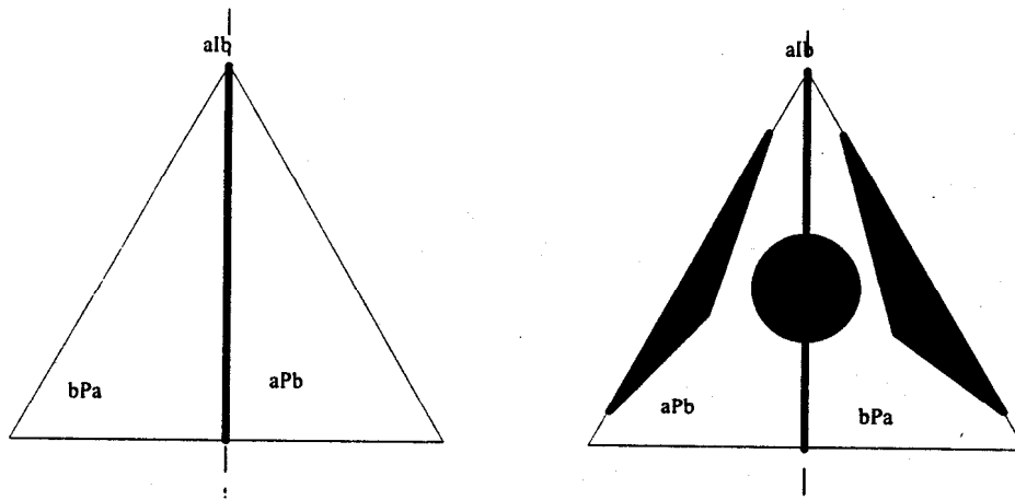
Figure 5. Examples of SWFs that satisfy Anonymity, Neutrality, and IIA
