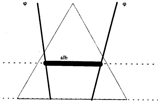
Figure 11. Illustration of \varphi -Indifference
