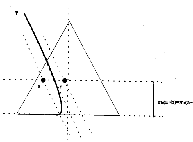
Figure 8. Illustration of \varphi -Weak I -Mon
