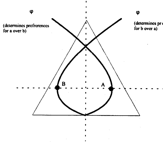
Figure 12. Characterization of SWF with a finite number of agents
