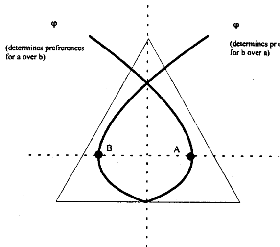
Figure 9. Illustration of \varphi -Weak I -Mon
