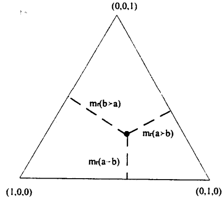
Figure 1. Graphical representation of a SWF that satisfies Anonymity and IIA
