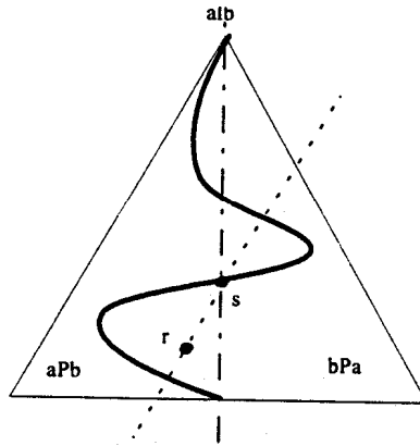
Figure 7. A SWF satisfying Weak I -Mon but not PR
