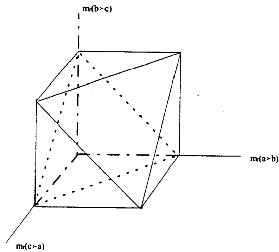
Figure 14. The truncated cube
