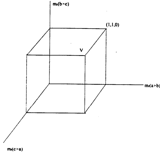
Figure 13. The unit cube
