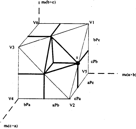
Figure 17. Majority rule in the truncated cube
