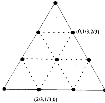
Figure 2. Domain for the case of \#A = 3
