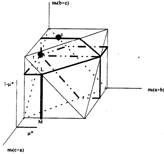
Figure 20. Graphical illustration of Arrow's Theorem
