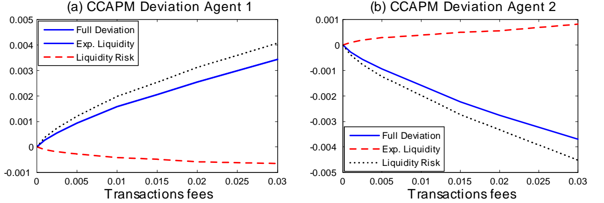
Figure 12: CCAPM deviations. The panels show the average (across paths and dates) of deviations from the classic consumption CAPM, computed using results up to period 25 for different levels of transactions fees, in the range from 0% to 3%. The “expected liquidity” component is \mathbb{E}_t[\tau_{l,t+1,i}] ; the “liquidity risk” premium component is cov_t\left[\tau_{l,t+1,i}, \frac{\phi_{l,t+1}}{\mathbb{E}_t[\phi_{l,t+1}]}\right] . All parameters and variables are set at their benchmark values indicated in table 1.
