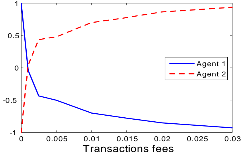
Figure 14: Average conditional correlation between the LIQ variable and the shadow liquidity variable \tau . The computation uses results up to period 25 for different levels of transactions fees, in the range from 0% to 3%. All parameters and variables are set at their benchmark values indicated in table 1. We use 20,000 simulations along the tree.
