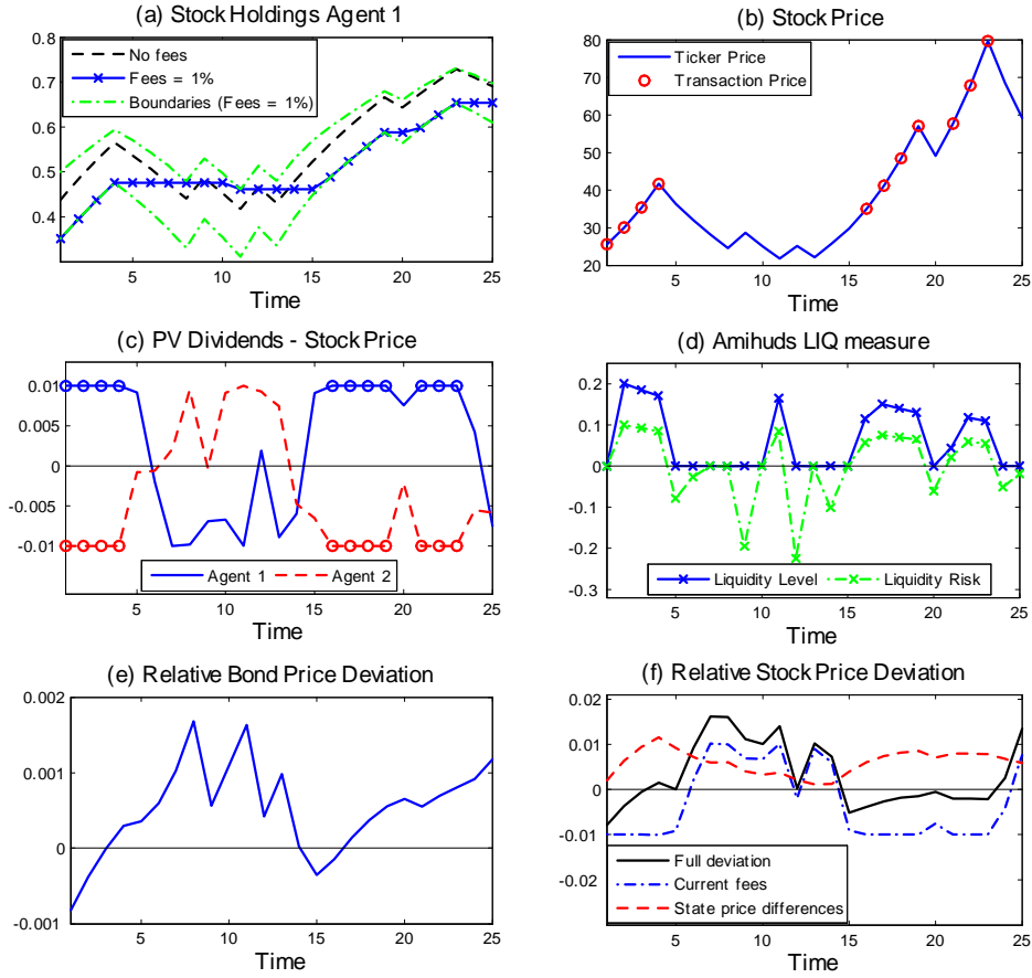
Figure 5: Sample time paths of stock holdings, the stock price and the difference between the stock price and each investor's value of the present value of dividends. Panel (a) shows stock holdings of the first agent along the paths for zero and 1% transactions fees. All parameters and variables are set at their benchmark values indicated in Table 1 (time-0 holdings (0,0) for agent 1). Panel (b) shows the stock ticker price along the sample path for 1% transactions fees. Panel (c) shows the present values of future dividends from the points of view of the two agents along the same path. Transactions are highlighted by a circle. Panel (d) shows Amihud's LIQ measure along the same path as well as its unanticipated or permanent component (marked Liquidity Risk). Panel (e) shows the relative deviation between the asset price in a zero-transactions fees economy and an economy with transactions fees along the same path. Panel (f) shows the components of the difference between the stock price in a zero-transactions fees economy and an economy with transactions fees, along the same path.
