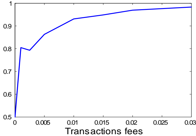
Figure 7: Serial dependence of trades : the frequency (across paths and dates) of a buy transaction following a previous buy transaction. All parameters and variables are set at their benchmark values indicated in table 1. We use 20,000 simulations along the tree. In each, the first 25 periods only are used.
