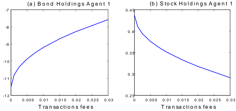
Figure 2: Optimal “exiting” holdings \theta of the securities. Optimal bond and stock holdings of the first agent for different levels of transactions fees, in the range from 0% to 3%. All parameters and variables are set at their benchmark values indicated in Table 1 (entering holdings (0, 0) ).
