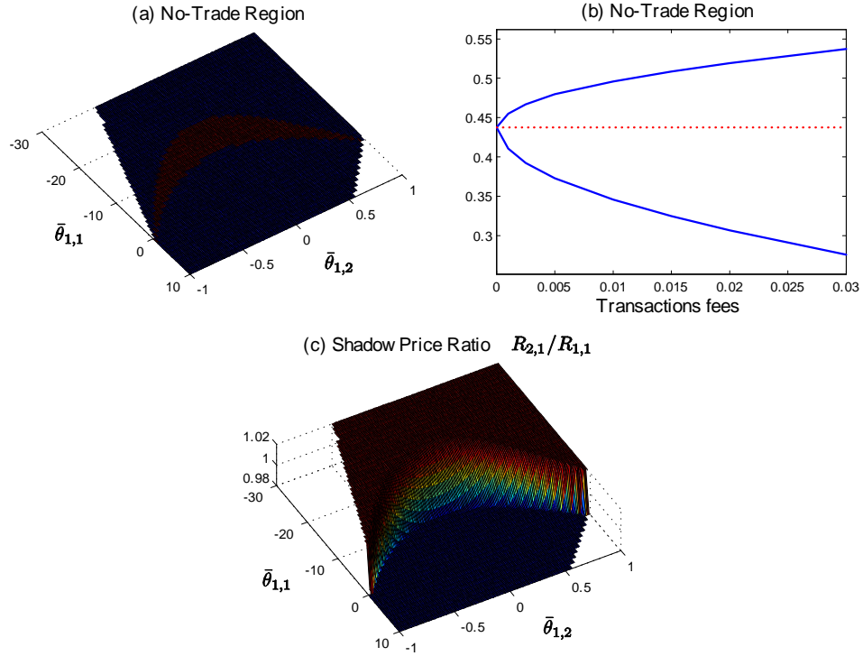
Figure 1: Equilibrium no-trade region. Panel (a) shows the no-trade region for different “entering” positions \bar{\theta} of the agents. Transactions fees are equal to 1\% \times value of shares traded, while Panel (c) displays the ratio of shadow prices across the trade and no-trade regions. Panel (b) shows the no-trade region for different levels of transaction fees from 0% to 3%. Consumption shares are set at the value corresponding to the initial holdings of Table 1. In all panels, parameters are as in Table 1.
