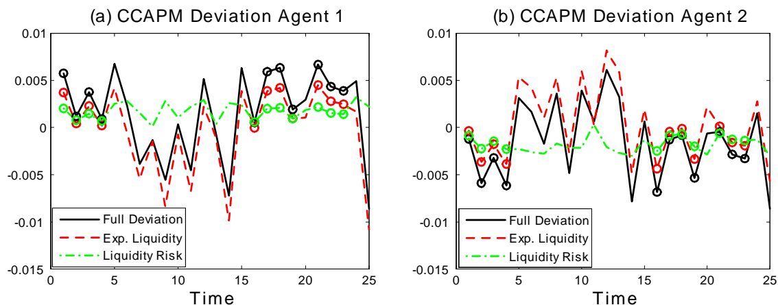
Figure 13: Fluctuations of the components of the deviations from the classic CCAPM , along the same sample path as in figure 5.
