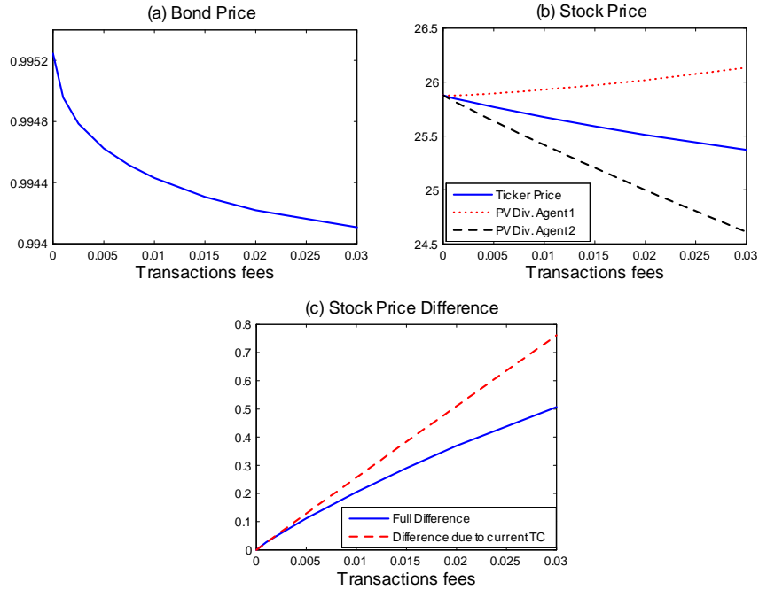
Figure 4: Initial asset prices. Panel (a) shows the initial period's bond price for different levels of transactions fees in the range from 0% to 3%. All parameters and variables are set at their benchmark values indicated in Table 1 (entering holdings (0,0) for agent 1). Panel (b) shows the initial period's stock price and the two agents' present values of dividends \hat{S}_{t,i,l} for different levels of transactions fees. Panel (c) shows the difference between the initial stock price in an economy with transactions fees and the stock price in economies without transactions fees. In addition, we show the component of the stock price difference that is due to the current amount of transactions fees.
