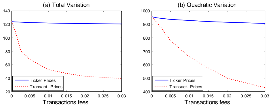
Figure 8: Total and quadratic variations of stock price depending on transactions fees . Panel (a) shows the total variation (defined in footnote 28) up to period 25 for different levels of transactions fees, in the range from 0% to 3%. All parameters and variables are set at their benchmark values indicated in table 1. We use 20,000 simulations along the tree. Panel (b) shows the quadratic variation computed the same way.
