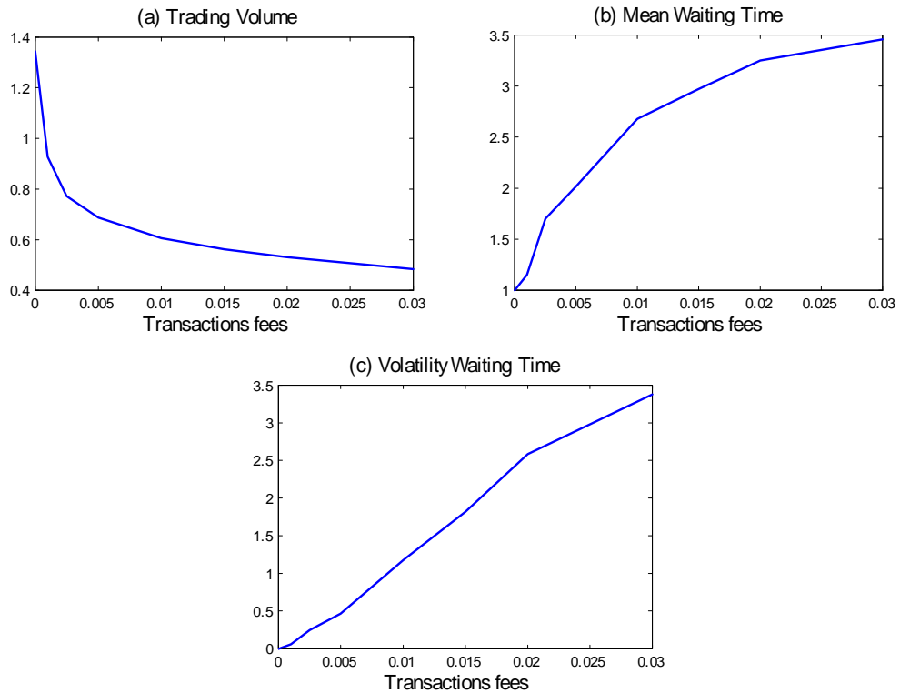
Figure 6: Trading volume and waiting time against transactions fees. Panels (a) and (b) show the average (across paths and dates) stock trading volume/year and the average waiting time between trades (measured in years) respectively, up to period 25 for different levels of transactions fees, in the range from 0% to 3%. Panel (c) shows the standard deviation of the waiting time calculated the same way. All parameters and variables are set at their benchmark values indicated in Table 1. We use 20,000 simulations along the tree. Panel (c) shows the standard deviation of waiting time computed the same way.
