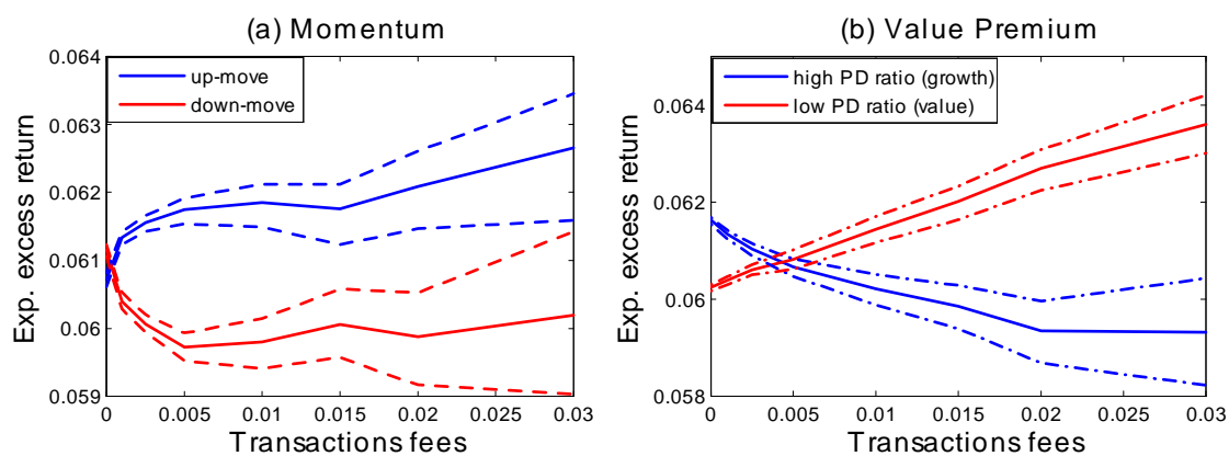
Figure 11: Short-term momentum and value premium in ticker price returns. Panel (a): from 20,000 simulations we sort the events, or nodes visited by a path, into two groups (dubbed “up” and “down” move) based on their last period return (realized return above or below the ex ante conditional return). Panel (b): we sort simulation events into those that are below and above the mean, according to their price/dividend ratio. The curves show the one-period ahead conditional expected return of the two groups of events. The computation is done on the first 25 periods of the tree. The dashed lines show the interval of two standard deviations across paths. All parameters and variables are set at their benchmark values indicated in Table 1.
