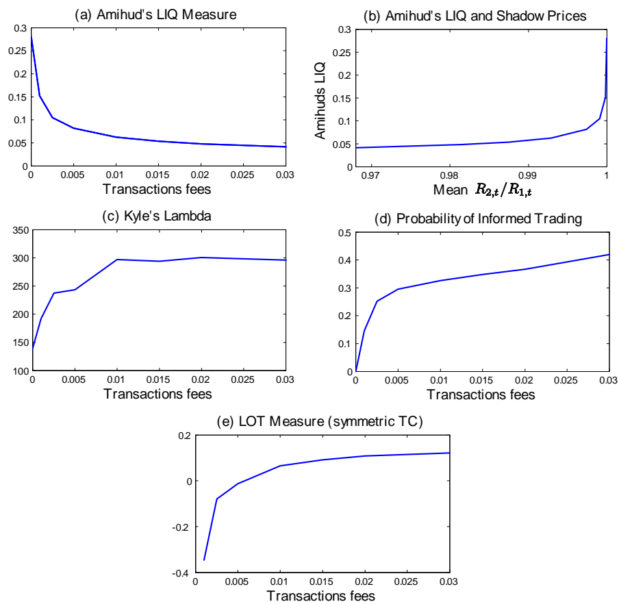
Figure 9: Liquidity variables. The first two panels show the average across paths and dates of Amihud's LIQ measure, computed using simulated results up to period 25 for different levels of transactions fees, in the range from 0% to 3% (Panel (a)) and against the average shadow price ratio (Panel (b)). All parameters and variables are set at their benchmark values indicated in table 1. We use 20,000 simulations along the tree. Panel (c) shows Kyle's lambda and computed in the same way using Madhavan-Smidt regression. Panel (d) shows the average PIN measure. Panel (e) shows the LOT/FHT measure based on frequency of no trade.
