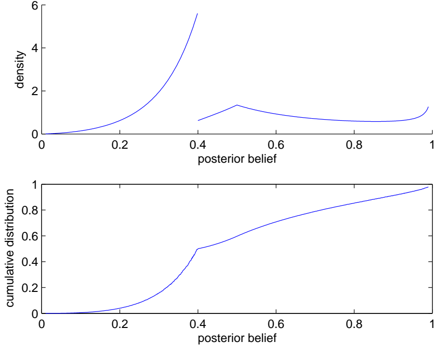
Figure 2: Equilibrium Distribution of Posterior Beliefs
