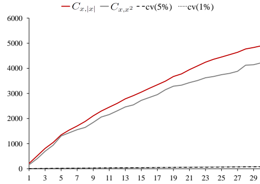
(b) C_{x,|x|,m} and C_{x,x^2,m} tests at lags m = 1, 2, \dots, 30 .
