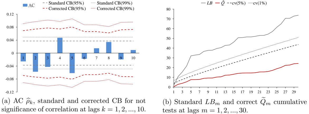
Figure 6: FTSE100 daily returns, 2008-2018. Correlogram
