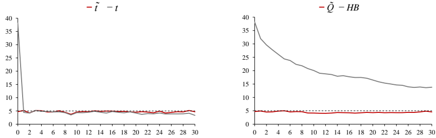
(b) x_t = \varepsilon_t, y_t = r_t^2, r_t = \sigma_t \varepsilon_t, \sigma_t^2 = 1 + 0.2r_{t-1}^2
