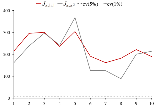
(a) J_{x,|x|,k} , J_{x,x^2,k} tests at lags k = 1, 2, \dots, 10 .
