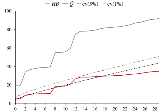
(b) Standard HB_{xy,m} and correct \tilde{Q}_{xy,m} cumulative tests at lags m = 0, 1, \dots, 30 .
