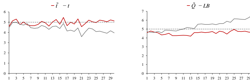
(a) x_t = \varepsilon_t
