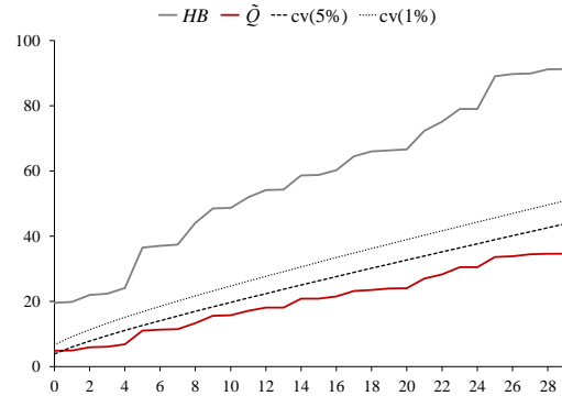
(d) Standard HB_{yx,m} and correct \tilde{Q}_{yx,m} cumulative tests at lags m = 0, 1, \dots, 30 .
