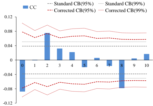
(a) CC \hat{\rho}_{xy,k} , standard and corrected CB for not significance of cross-correlation at lags k = 0, 1, \dots, 10 .
