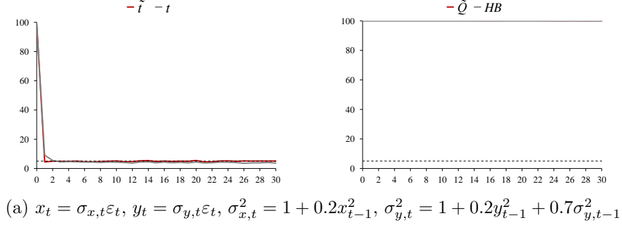
Figure 4: Power. Rejection frequency (in %) at \alpha = 5\% of corrected \tilde{t}_{xy,k} and standard t_{xy,k} tests (left) and corrected \tilde{Q}_{xy,m} and standard HB_{xy,m} cumulative tests (right) at lags k, m = 0, 1, \dots, 30 . \varepsilon_t, \eta_t \sim \text{iid } \mathcal{N}(0, 1) , \{\varepsilon_t\}, \{\eta_t\} independent.
