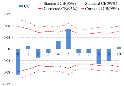
(c) CC \hat{\rho}_{yx,k} , standard and corrected CB for not significance of cross-correlation at lags k = 0, 1, \dots, 10 .
