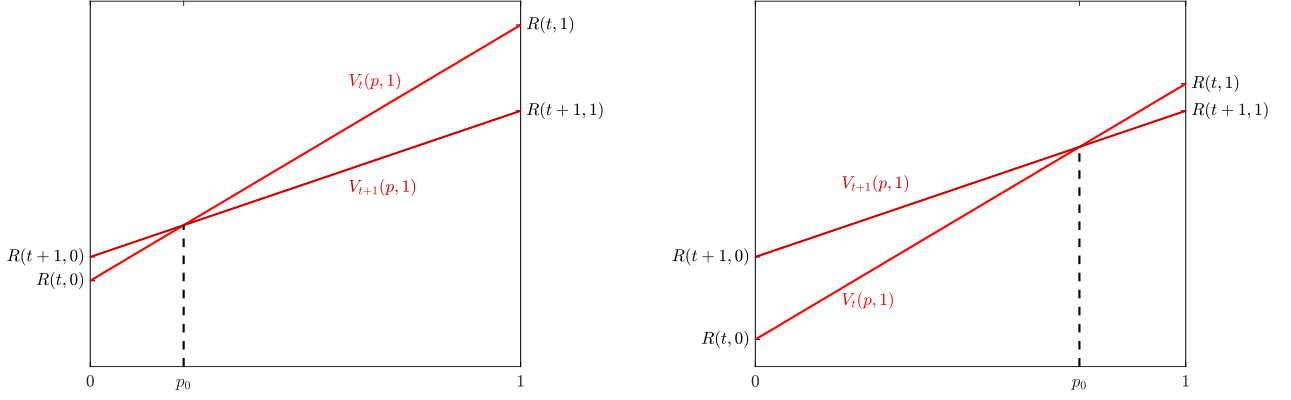
Figure 3: The value from acting in t and t + 1 under a low prior (left panel) and high prior (right panel).
