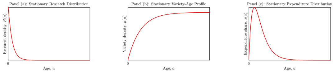
Figure D.4: The cross-sectional stationary distributions with \bar{\lambda} = 1 . Note: The figure presents the illustrative calibration discussed in Section 3.
