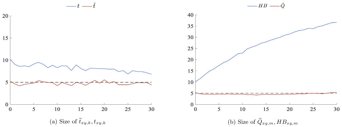
Fig. 9. Empirical sizes (in %) of tests \tilde{t}_{xy,k}, t_{xy,k} (left panel) and HB_{xy,m}, \tilde{Q}_{xy,m} (right panel). Nominal size \alpha = 5\% Model 4.5. (For interpretation of the references to color in this figure legend, the reader is referred to the web version of this article.)
