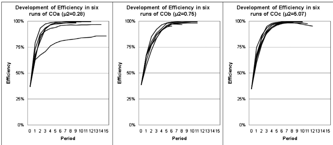
Fig. 4. Development of efficiency (in six independent runs for each default penalty with money and good carried over; Period 0 = autarky).
