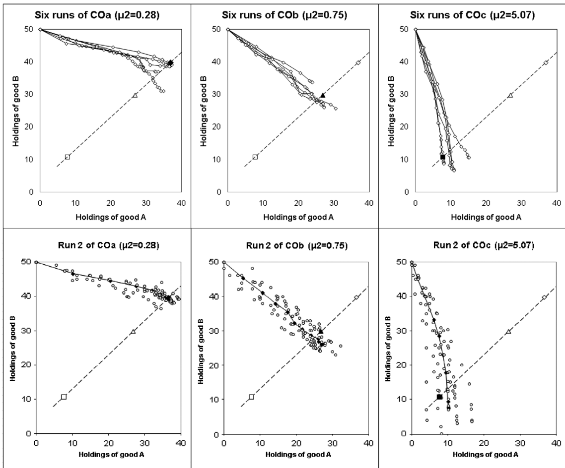
Fig. 2. Paths of holdings of goods A and B over periods in treatment CO (with goods and money balances carried over period-to-period). Top panels: Trader-type averages in six independent runs for each default penalty. Bottom panels: Trader-type average and individual holding details of run 2 for each default penalty.
