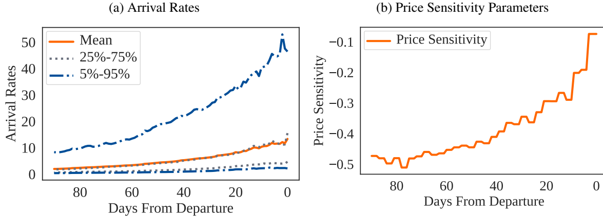
Figure 6: Arrival Rates and the Price Sensitivity Parameters
