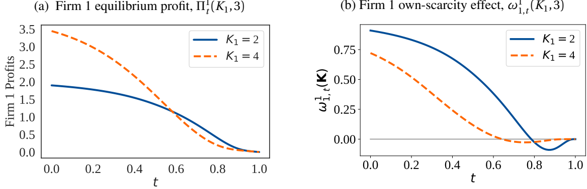
Figure 2: Simulated profits and own-scarcity effects when K_2 = 3 and K_1 varies
