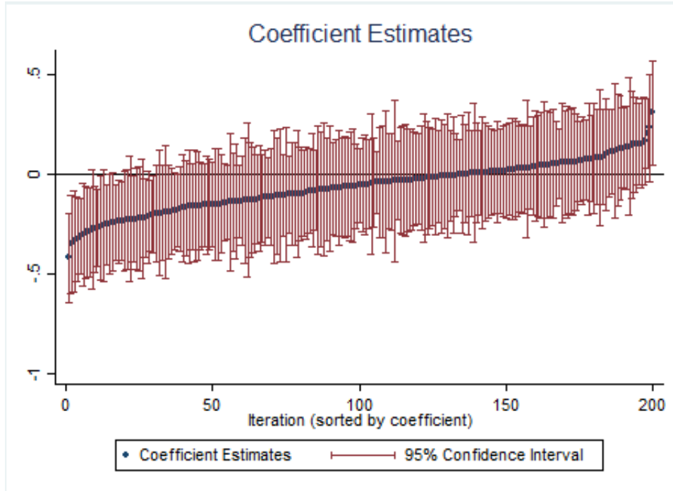
Figure 3: Coefficient estimates and 95% confidence intervals for 200 replications of the estimation exercise in column 12 of Table 4, where the main independent variable is the distance from a set of 10 randomly selected municipalities that (i) lie within 80 km of a near-Piedmontese community and (ii) have experienced no brigandage. Only 2 coefficients are positive and significant at 5% (3 at 10%).
