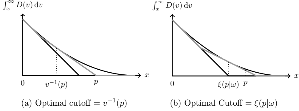
Figure 2: Optimal Cutoff
