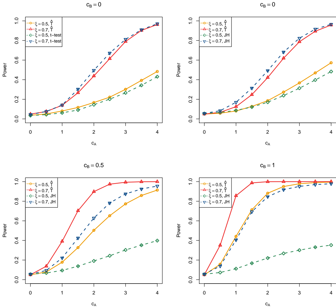
Figure C: Testing Parametric Form - Size-adjusted empirical power of our adaptive test \widehat{T}_n (solid lines), \xi = \{0.5, 0.7\} . First row: power comparison to the t -test and JH test when c_B = 0 ; Second row: power comparison to the JH test when c_B = 0.5 and c_B = 1 . Design from Section 5.2. Replication of Figure 2 with n = 1000 .
