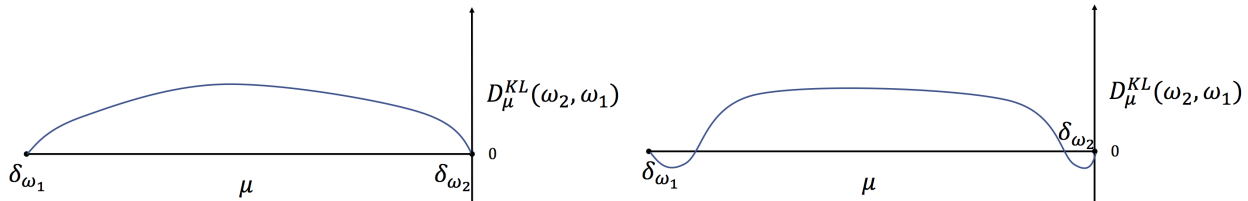
Figure 1: Prediction accuracy ranking of \omega_1 vs. \omega_2 as a function of \mu when \omega^* = \omega_1 . Left: \hat{\beta} = \beta . Right: \beta > \hat{\beta} . Here D_\mu^{\text{KL}}(\omega_2, \omega_1) := \text{KL}(P_\mu(\cdot|\omega^*), \hat{P}_\mu(\cdot|\omega_2)) - \text{KL}(P_\mu(\cdot|\omega^*), \hat{P}_\mu(\cdot|\omega_1)) .
