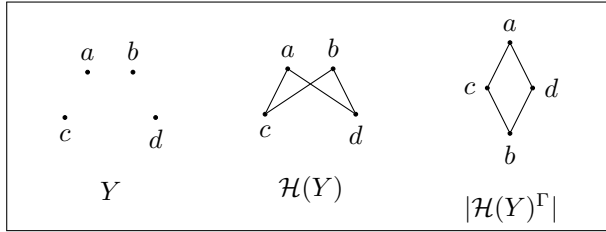
FIGURE 2. Example of a set that cannot compose a hulling
