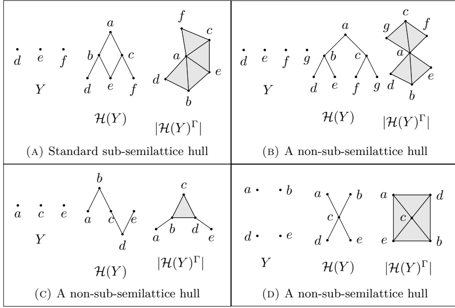
FIGURE 1. Examples of sets \mathcal{H}(Y) \in \mathcal{H}
