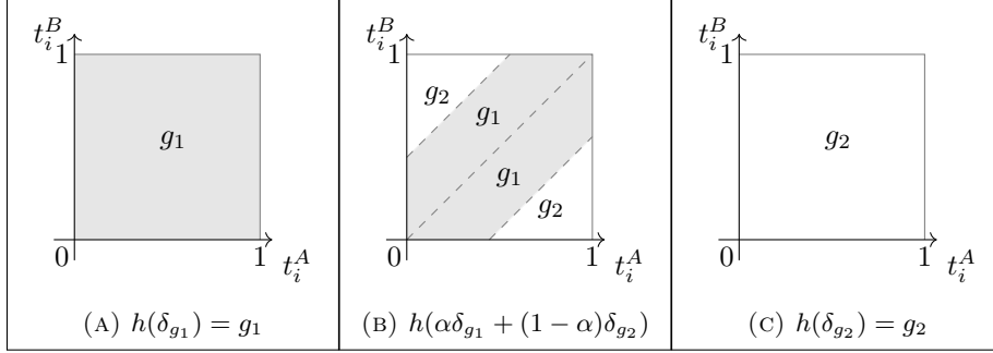
FIGURE 3. Piecewise composition of the monotone realization h(|(g_1, g_2)|)
