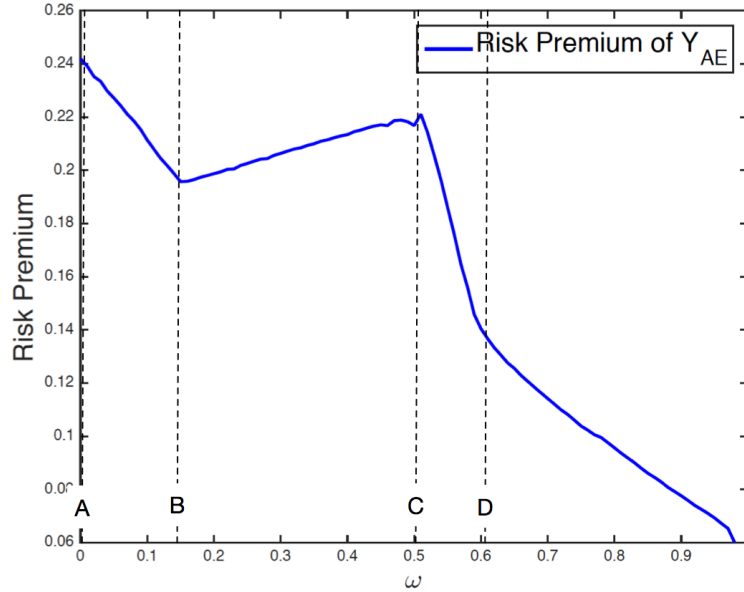
Figure 16: Effects of QE on the Risk Premium of Y_{AE}
