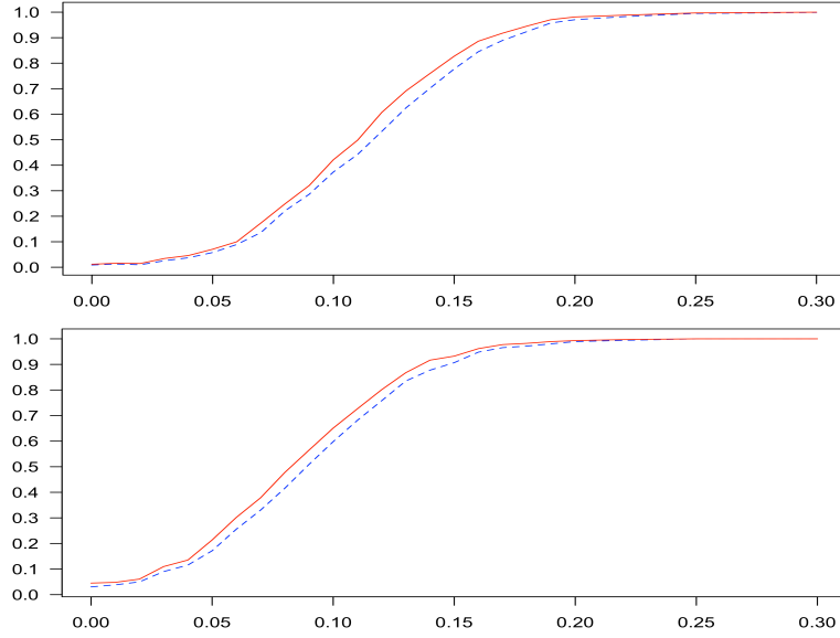
FIGURE 7.1.— Rejection probabilities at 1% (upper panel) and 5% level (lower panel) of the null hypothesis as a function of r = \phi(h_0) for the SQLR (solid red line) and for the bootstrap SQLR (dashed blue line) for NPQIV.
