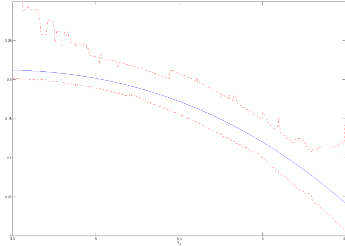
FIGURE 7.III.— PSMD Estimate of the NPQIV food-in Engel curve (blue solid line), with the 95% pointwise confidence bands (red dash lines).
