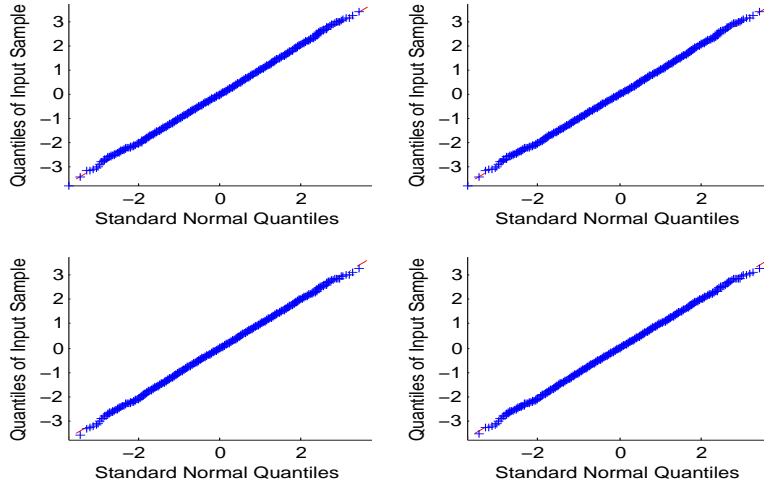
FIGURE 7.II.— QQ-Plot for t tests \hat{t}_j for j = 1, 2 for a linear functional (first row) and a nonlinear functional (second row) of NPIV, with q^{k(n)} = Pol(4) and p^{J_n} = Pol(16) .
