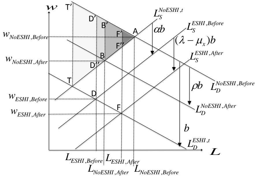
Figure 1: Graphical Model
