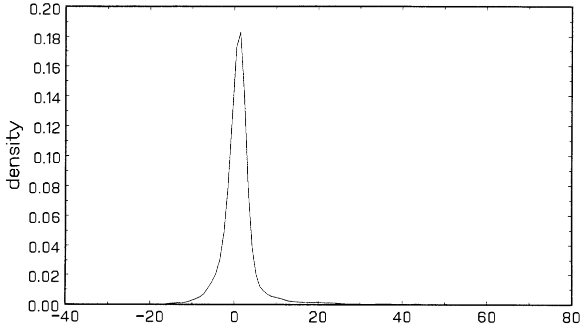
Figure 5(b): Sampling Distribution 10-period ahead OLS Impulse Responses
