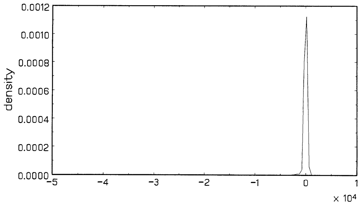
Figure 5(b): Sampling Distribution 10-period ahead OLS Impulse Responses
